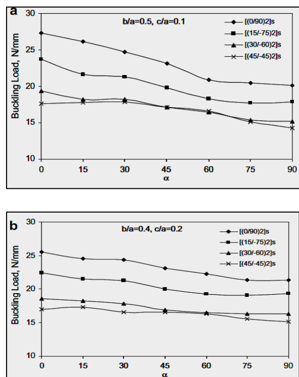
Fig. 3. The Effect of Parameter on Buckling Load [8]
